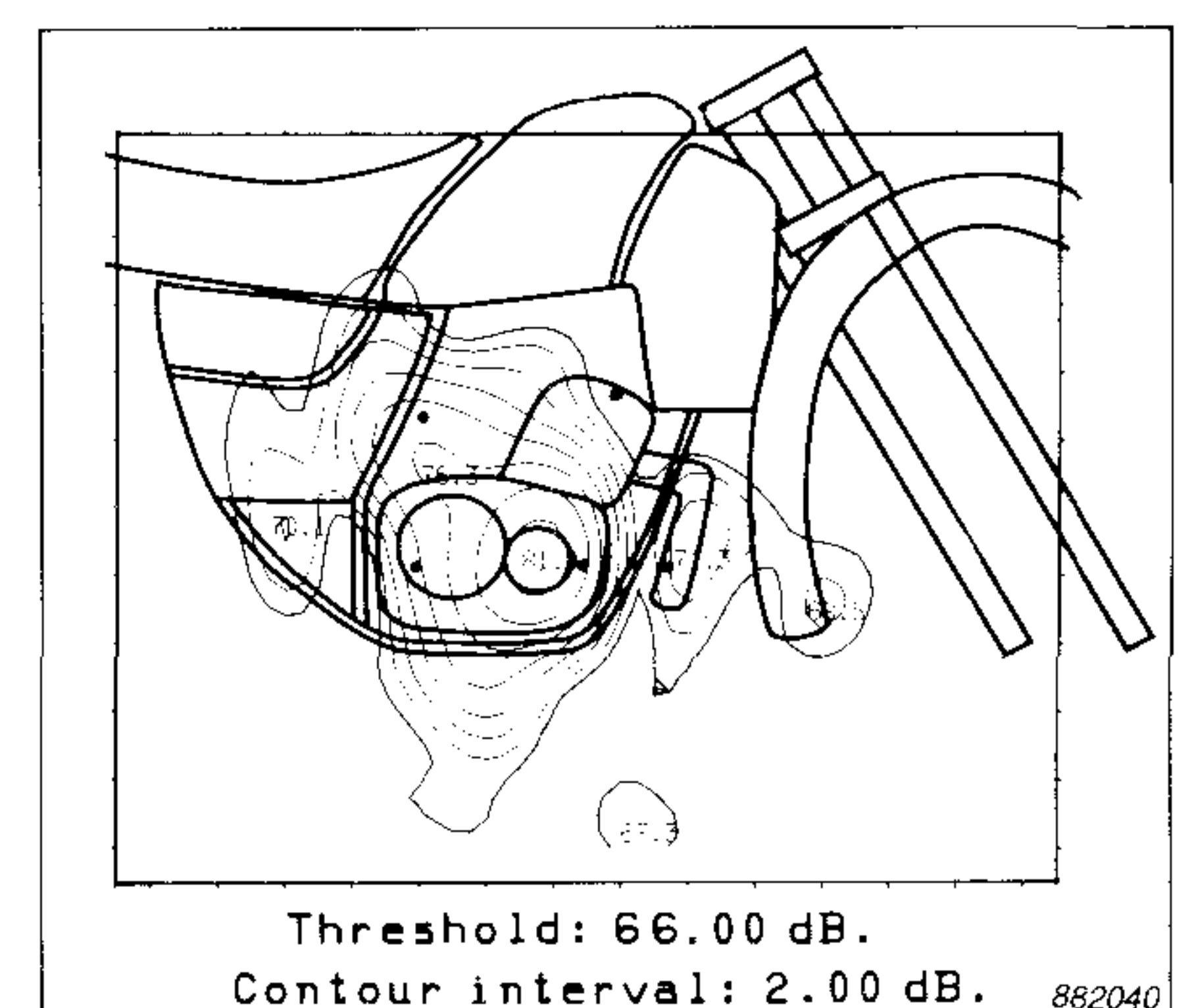
Fig. 7. Pressure contour plot. 1600 Hz twelfth octave band
