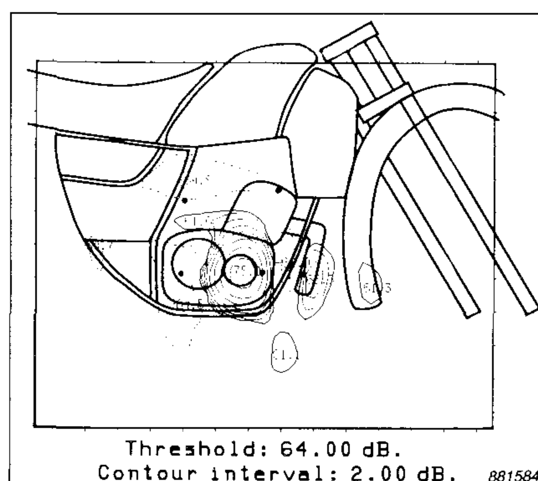
Fig. 6. Reactive intensity plot. 1600 Hz twelfth octave band
