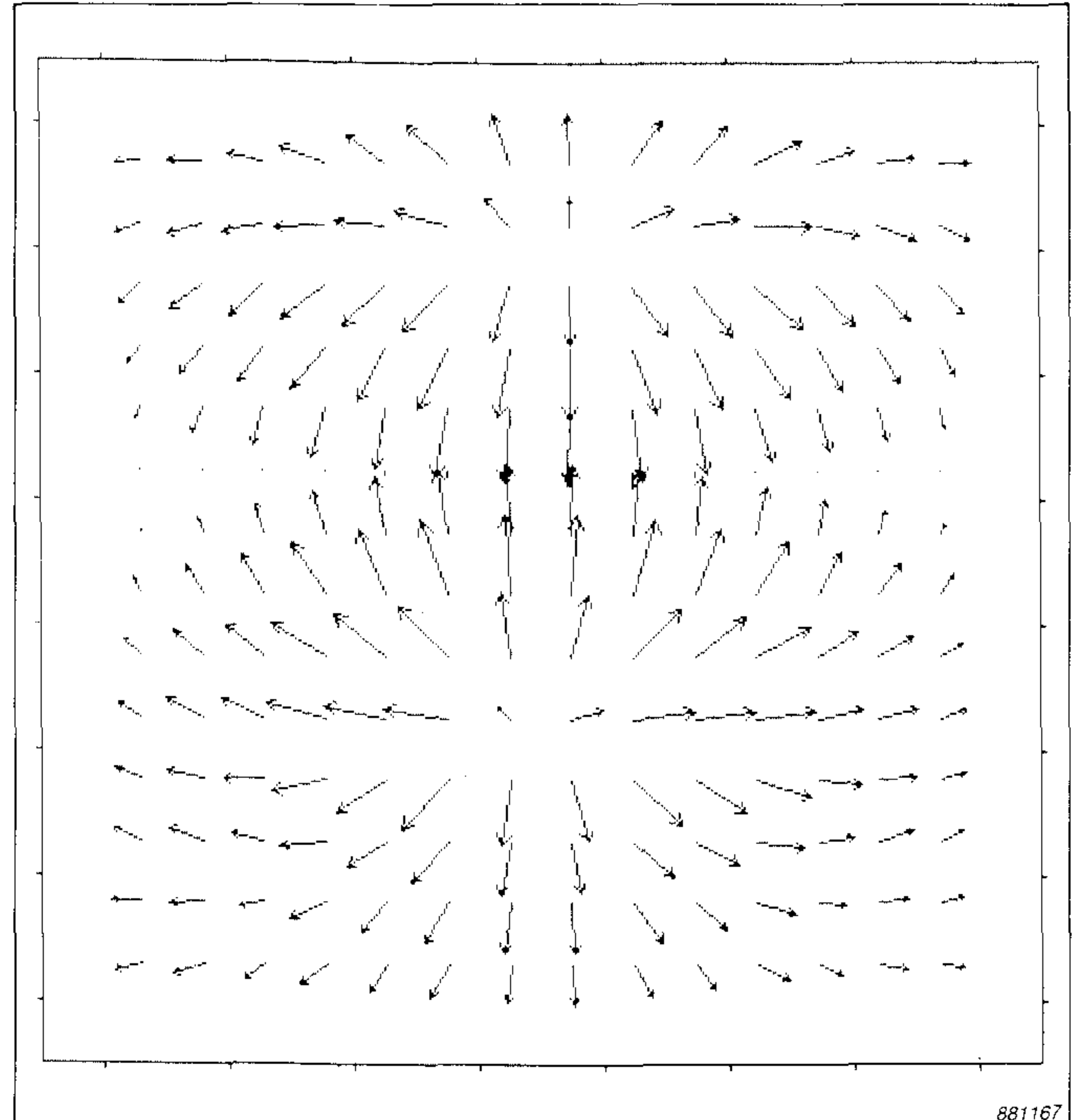
Fig. 2. Reactive intensity vector plot over the same loudspeakers as in Fig. 1. The location of the loudspeakers can clearly be seen
