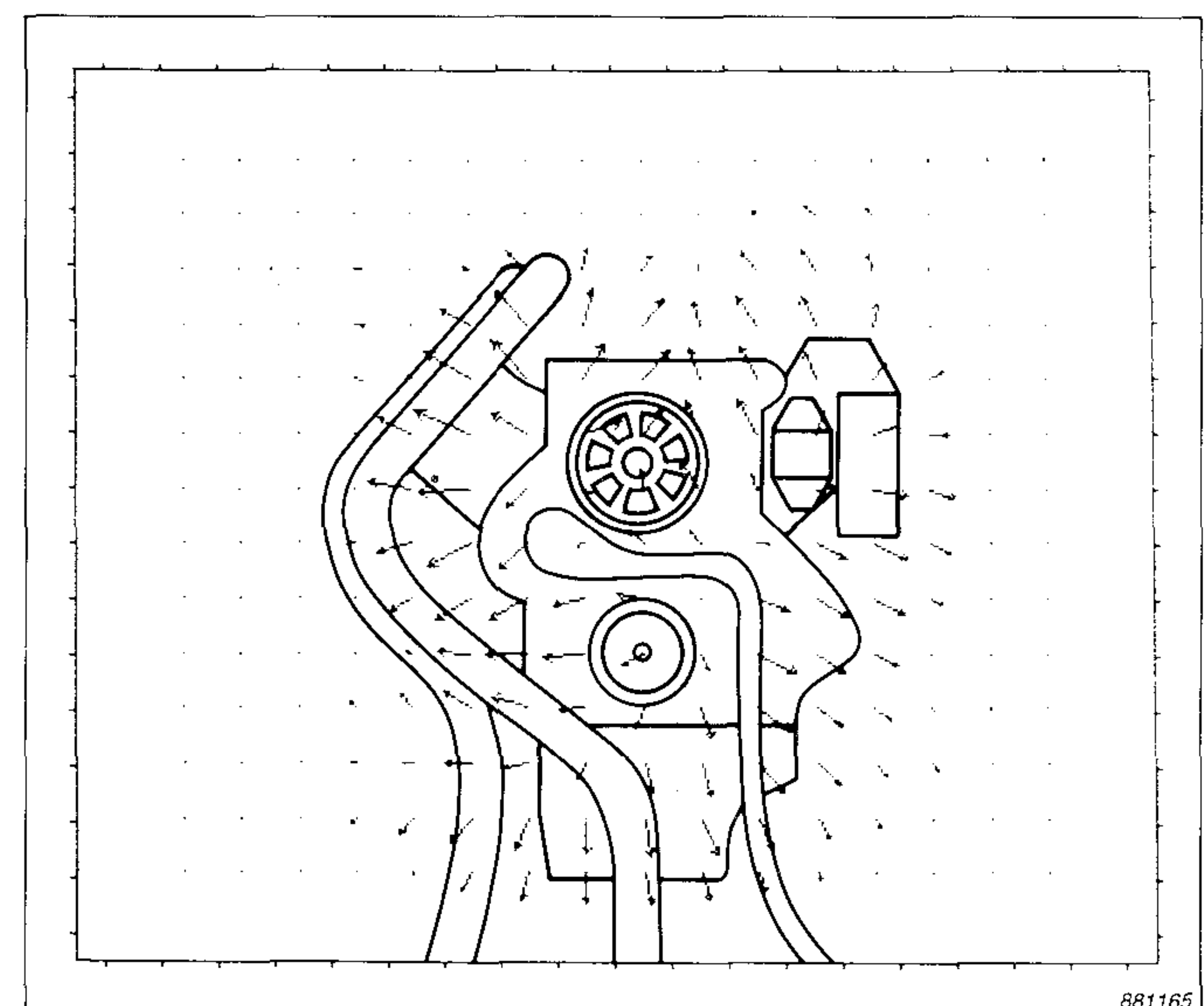
Fig. 4. Reactive intensity vector plot. 400 Hz third octave band
