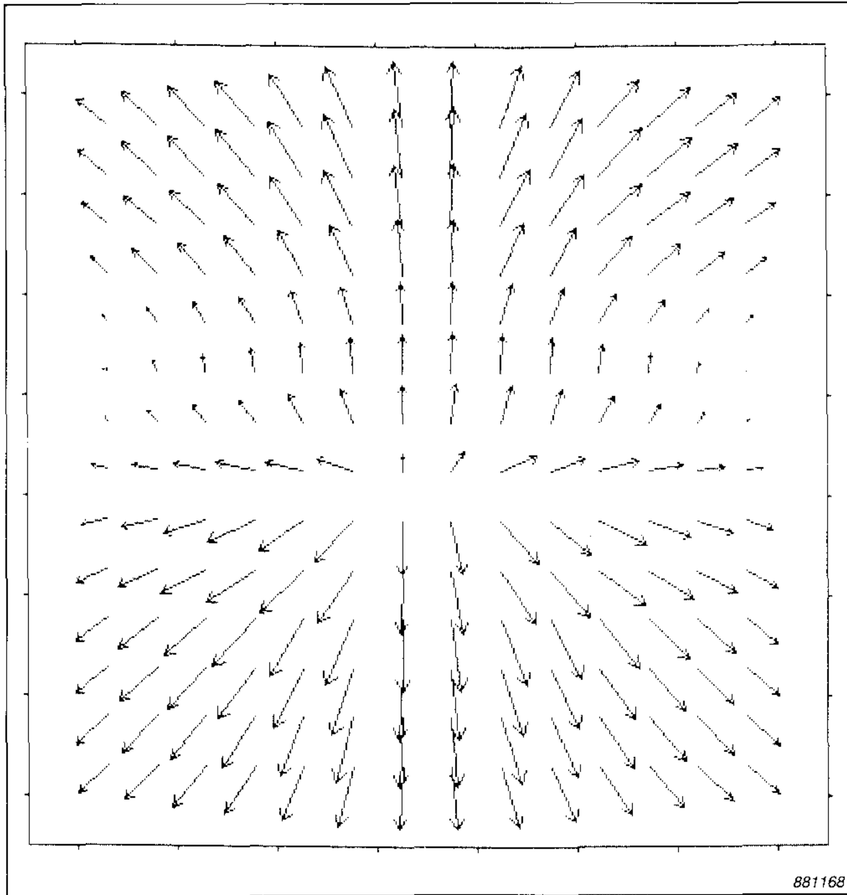
Fig. 1. Active intensity vector plot over two loudspeakers in anti-phase. The location of the loudspeakers is not obvious
