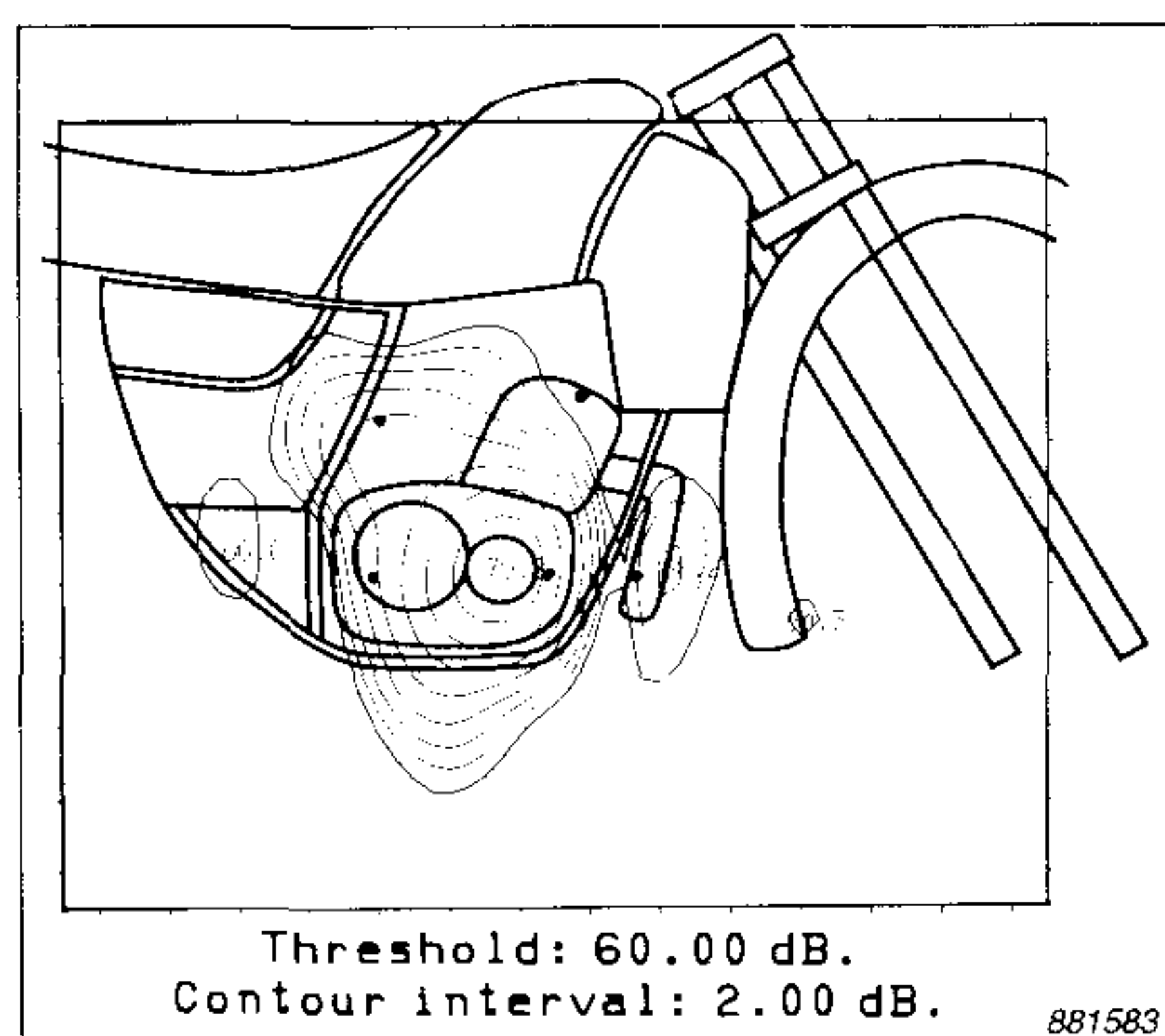
Fig. 5. Active intensity contour plot. 1600 Hz twelfth octave band
