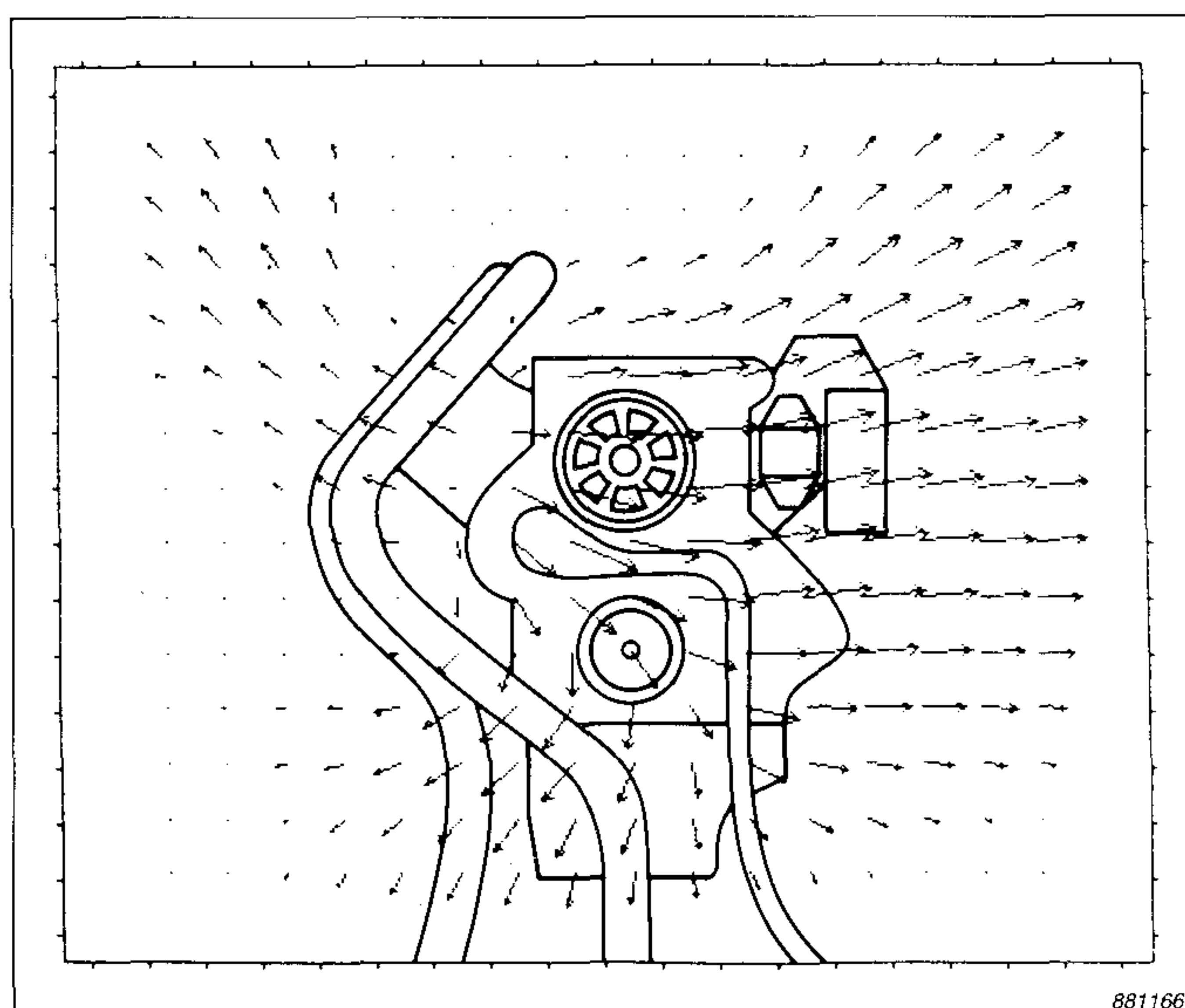
Fig. 3. Active intensity vector plot. 400 Hz third octave band
